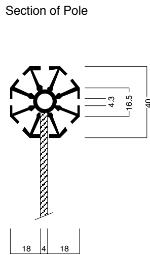
Specification of pole, beam, joint
